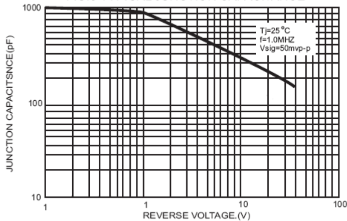
FIG.5-TYPICAL JUNCTION CAPACITANCE
