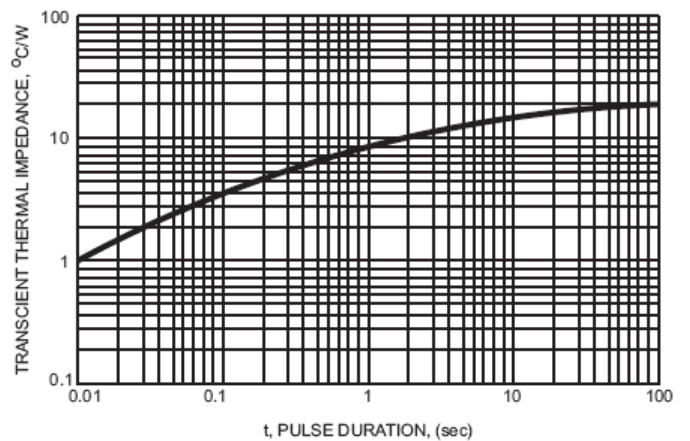
FIG.6- TYPICAL TRANSIENT THERMAL IMPDANCE
